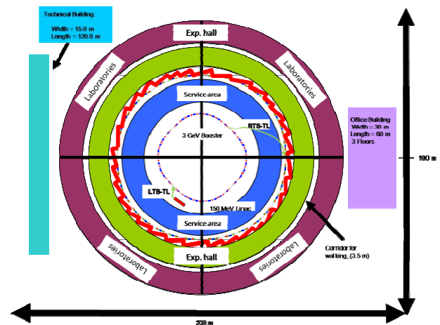
Figure 1: General layout of ILSF.
