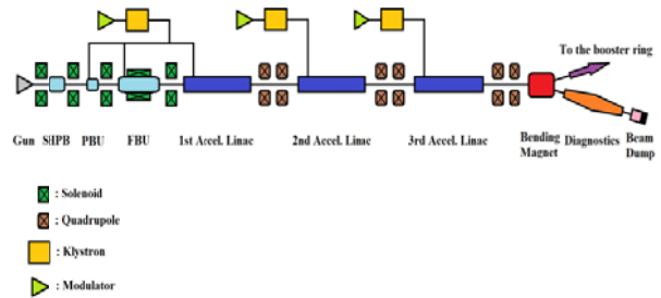
Figure4. Lattice layout of the pre-injector at ILSF.
