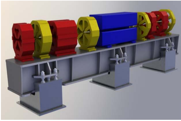
Figure3. Primary design of ILSF storage ring Girders of the Matching Cell.
