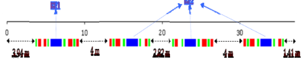
Figure 2: Arrangement of magnets in half a super-period of ILSF-Lattice-1. The blue arrows show the locations of dipole magnets.
