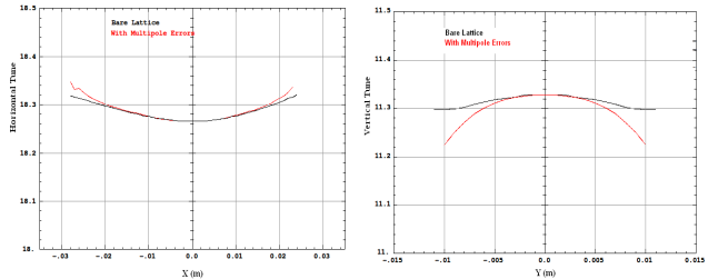
Figure 7: Tune shift with horizontal (left) and vertical (right) amplitude with and without multipole errors.
