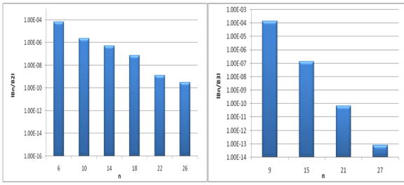
Figure 3: Absolute normalized multipoles errors for quadrupole magnets at the \pm 18 mm good field region (left) and sextupole magnets at the \pm 12 mm good field region (right).
