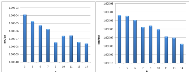
Figure 1: Absolute normalized multipoles errors for bending magnet BE1 (left) and BE2 (right).
