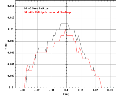
Figure 2: Dynamic aperture of ILSF ring for two cases of without multipole errors and with multipole errors in dipoles.
