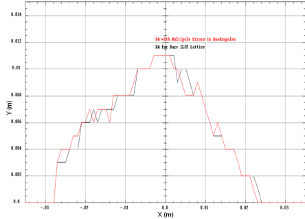
Figure 4: Dynamic aperture of ILSF ring for two cases of without multipole errors and with multipole errors in quadrupoles.
