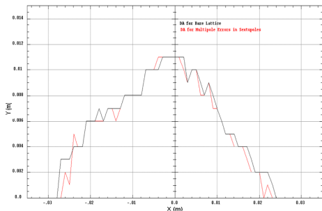
Figure 5: Dynamic aperture of ILSF ring for two cases of without multipole errors and with multipole errors in sextupoles.
