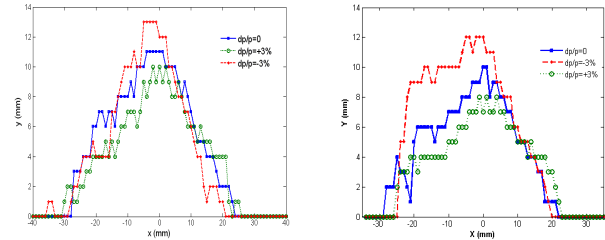
Figure 6: Dynamic aperture with multipole errors in all kind of magnets (left), and without any errors (right).
