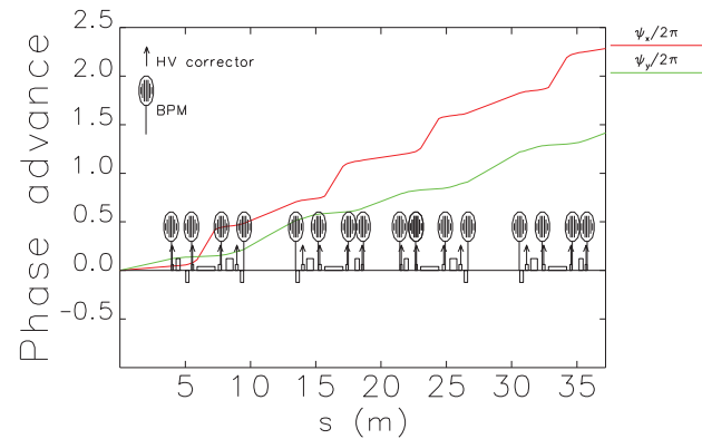
Figure 2. Location of the BPMs and the HV correctors in half a super period of the ring.
