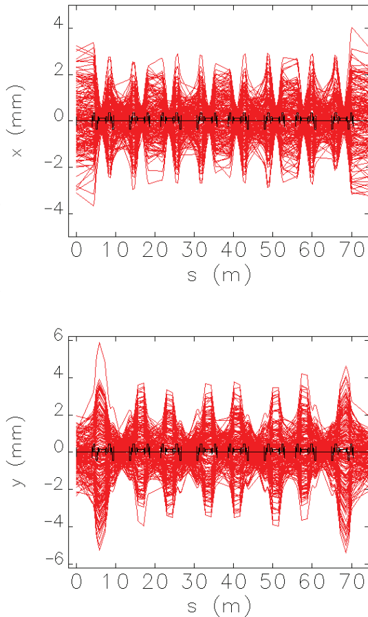
Figure 1. Distorted closed orbit in a super period of the storage ring for 200 seeds random errors, horizontal orbit (top), vertical orbit (bottom).
