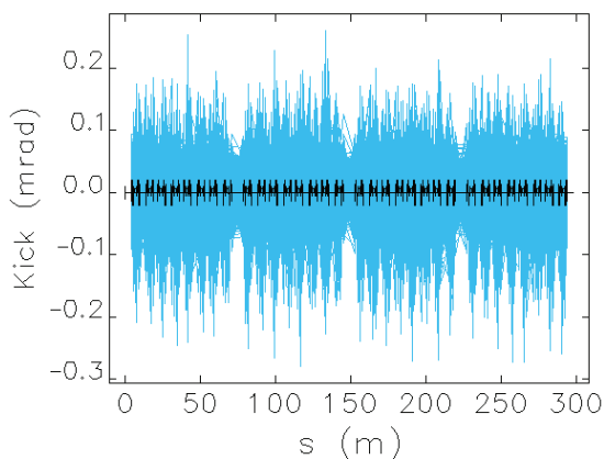
Figure 4. Strength of the corrector magnets in the ring for 200 seeds random errors.
