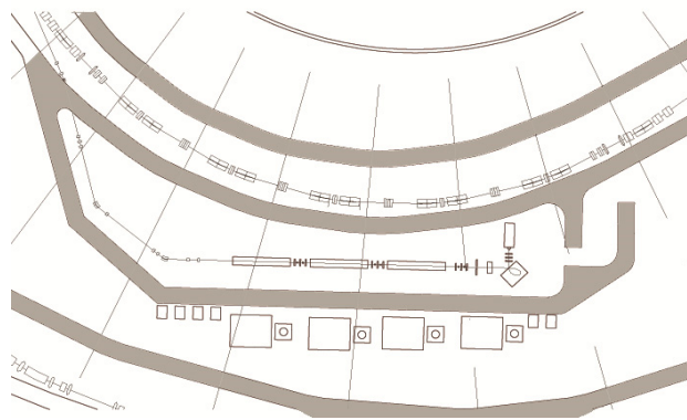
Figure 3. Mechanical drawing of the LTB line including shielding walls.
