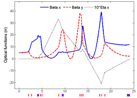
Figure 4. The optical functions along the LTB line with the initial Twiss functions of \beta_x=\beta_y=5 m and \alpha_x=\alpha_y=0 .
