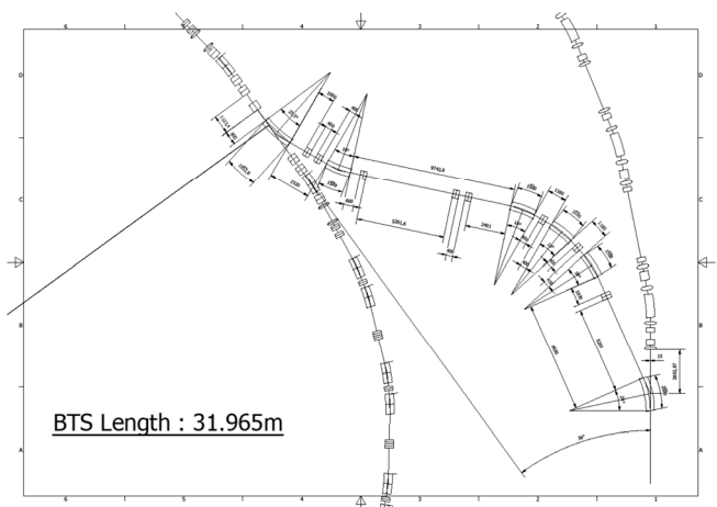
Figure 5. Mechanical drawing of the BTS line.
