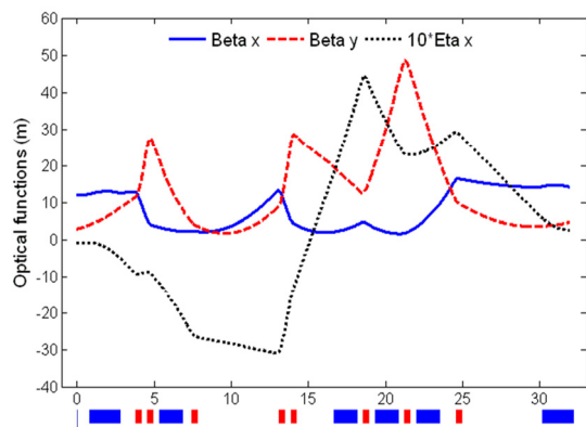
Figure 6. The optical functions along the BTS line with the initial and final Twiss functions given in Table 1.
