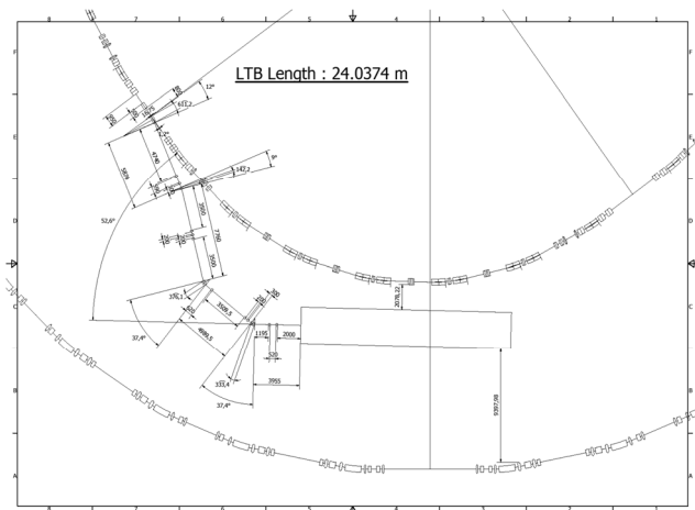
Figure 2. Mechanical drawing of the LTB line.
